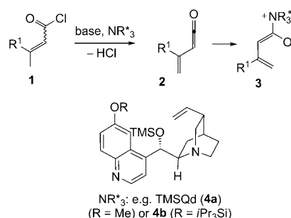
Scheme 1. Proposed formation of zwitterionic dienolate intermediates for [4+2] cycloaddition with aldehydes.
