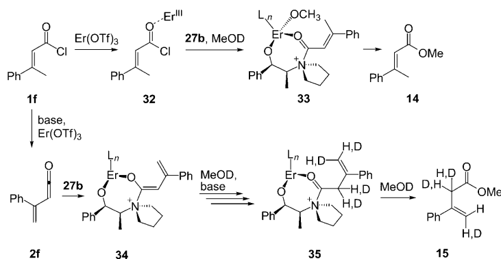
Scheme 15. General mechanistic alternatives, either through an acylammonium intermediate or through a vinylketene.
