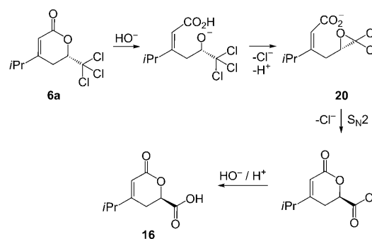
Scheme 11. Inversion of the configuration during the hydrolysis of 6a .
