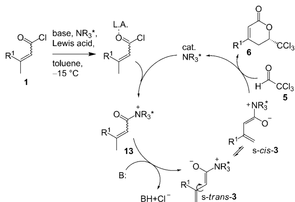
Scheme 6. Alternative I for the reaction mechanism, involving an acylammonium intermediate (L.A. = Lewis acid).
