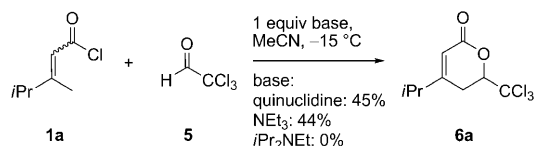
Scheme 2. Proof of concept.
