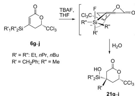
Scheme 13. Proposed explanation for the diastereoselectivity.
