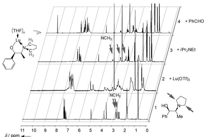
Figure 4. ^1\text{H} NMR complexation studies in [\text{D}_8]\text{THF} at RT. Spectrum 1: ligand 27b . Spectrum 2: ligand 27b + \text{Lu}^{\text{III}} triflate (1:1). Spectrum 3: ligand 27b + \text{Lu}^{\text{III}} triflate + i\text{Pr}_2\text{NEt} (1:1:1). Spectrum 4: ligand 27b + \text{Lu}^{\text{III}} triflate + i\text{Pr}_2\text{NEt} + \text{PhCHO} (1:1:1:1).
