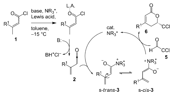
Scheme 7. Alternative II for the reaction mechanism, involving a vinylketene intermediate (L.A. = Lewis acid).
