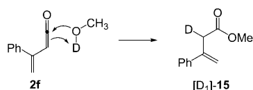
Scheme 8. Generation of monodeuterated ester [D_1] - 15 via a vinylketene intermediate.
