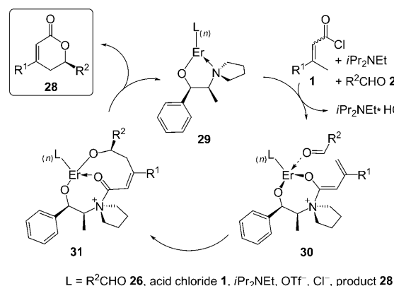
Scheme 14. Proposed catalytic cycle for the Er III -/amino-alcohol-catalyzed formation of \delta -lactones from \alpha,\beta -unsaturated acid chlorides 1 and aldehydes 26 .
