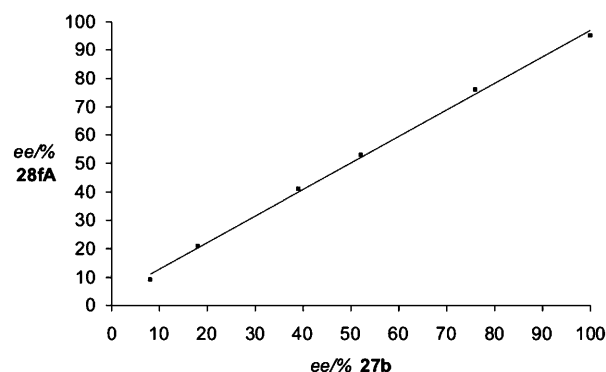
Figure 2. Investigation of a potential nonlinear effect for the formation of 28fA under the conditions of Table 10, entry 6.
