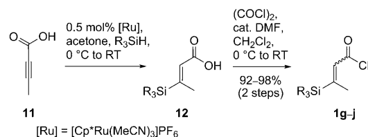
Scheme 4. Preparation of \alpha,\beta -unsaturated acid chlorides 1g–j bearing silyl substituents at their \beta -positions.
