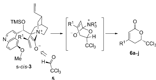
Scheme 5. Proposed explanation of the remote stereocontrol.
