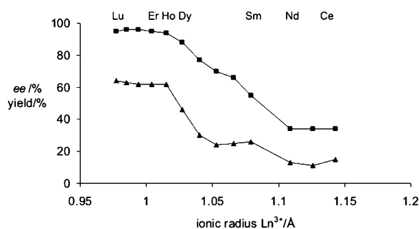
Figure 3. Influence of the ionic radius of \text{Ln}^{\text{III}} on the title reaction [data from Table 12; square: ee (%), triangle: yield (%)].
