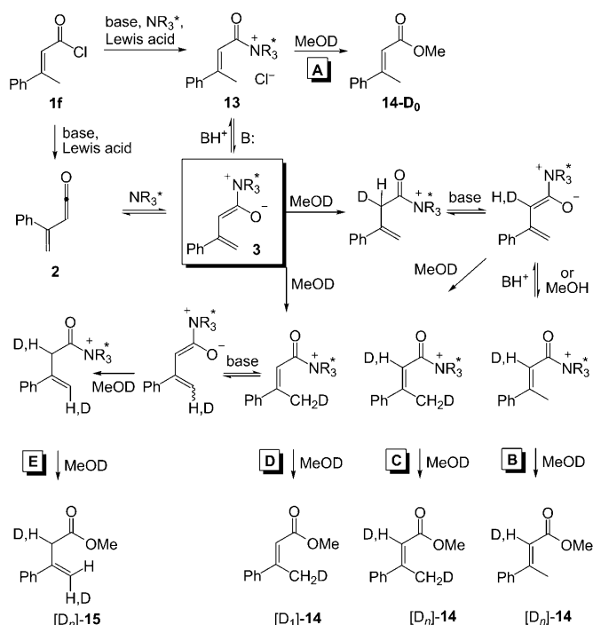
Scheme 9. General mechanistic picture of the equilibria involving the acylammonium/dienolate couple.
