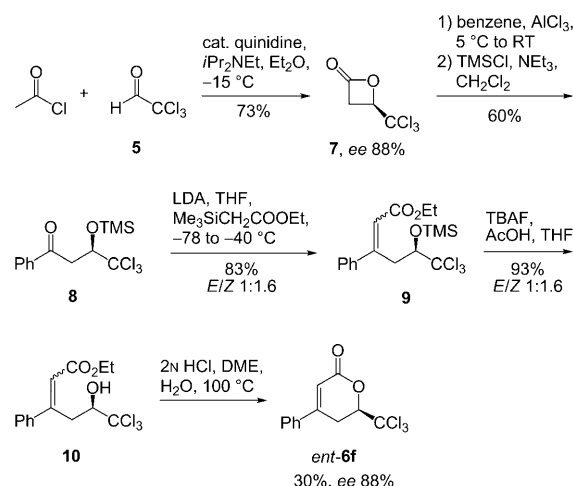
Scheme 3. Determination of the absolute configuration by chemical correlation: synthesis of ent - 6f via the known \beta -lactone 7 .
