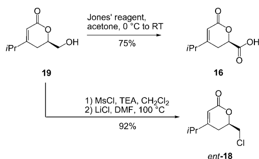
Scheme 12. Determination of the absolute configuration of the stereocenter by chemical correlation.
