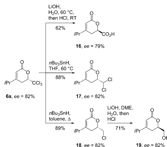
Scheme 10. Synthetic modification of the trichloromethyl group.
